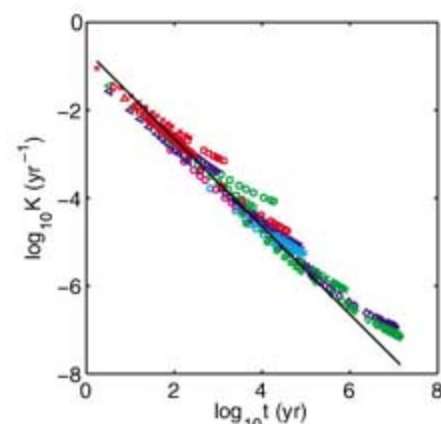
Fig. 4. The effective time-dependent reactivity K(t) = -d \ln g/dt . Symbols: K computed from Eq. 5, with estimates of k_{\min} obtained from the fits of Fig. 2. Symbols and colors in both figures correspond to the same cores. Straight line: the theoretical approximation K \cong 0.23 \times t^{-1} of Eq. 5, obtained without any free parameters. The rightward trends away from the line represent the slowing of rates as t approaches k_{\min}^{-1} .
